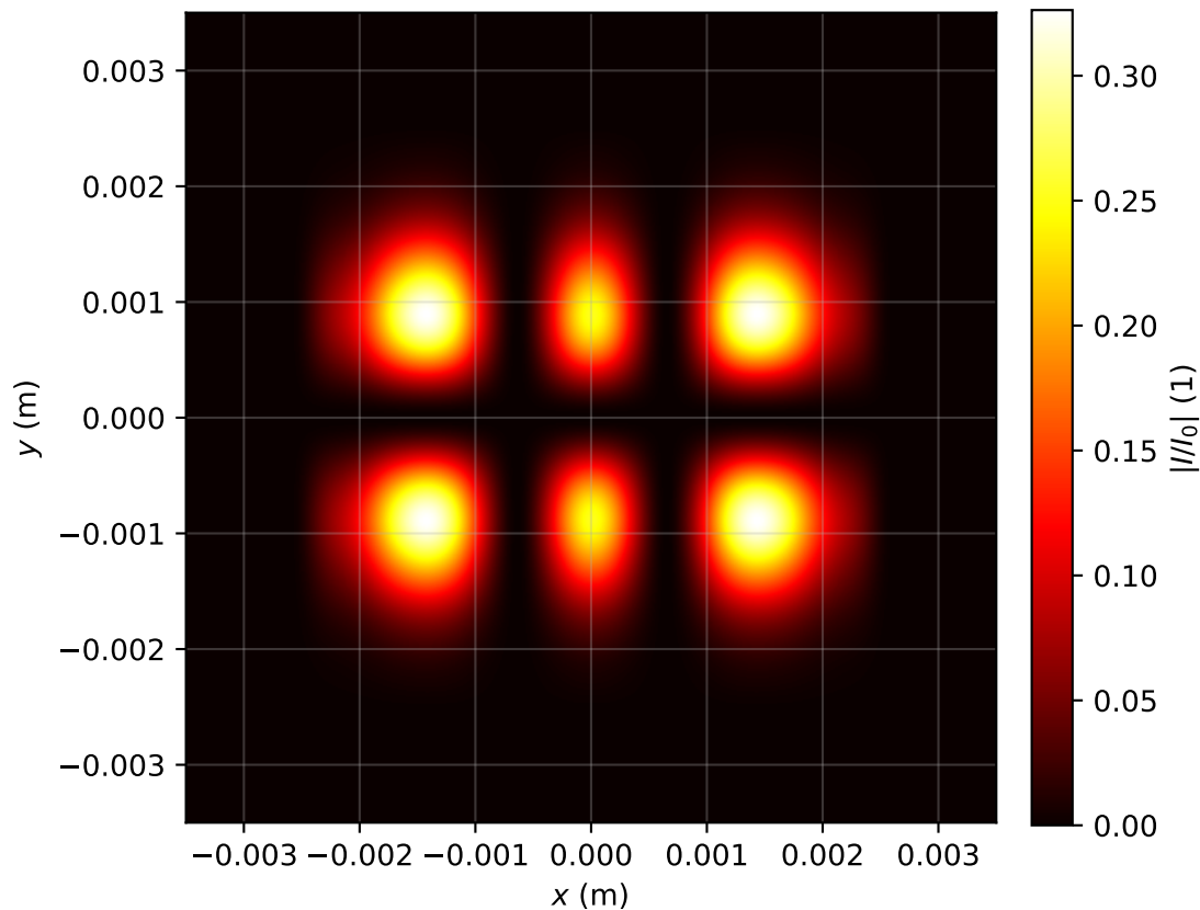
Intensity profile I(x, y, z = 3.025)/I_0 , P_{in}=0.5P_{cr} , artificial time
